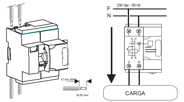
REC2C - output contact
