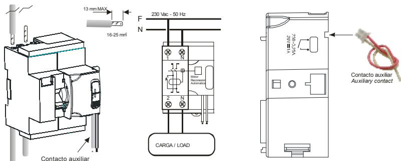
REC2C - output contact
